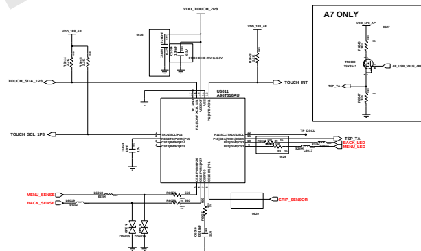
Touch Key + Grip Sensor
